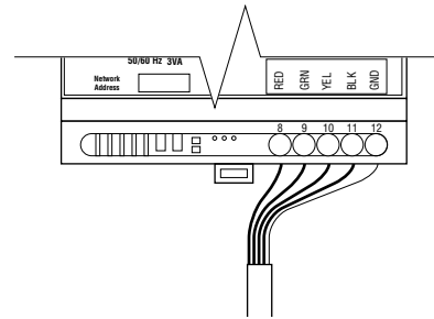
Figure 6. Sensing Cable Connections
