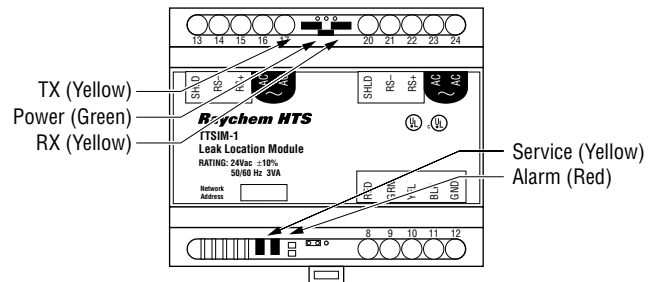
Figure 10. LED Locations
