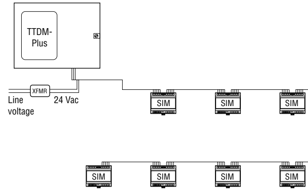
Figure 3. Power Supply to SIM units
