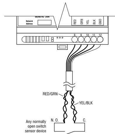
Figure 7 Switch Type Sensor
