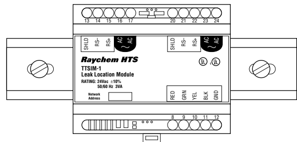
Figure 1. DIN Rail Mount
