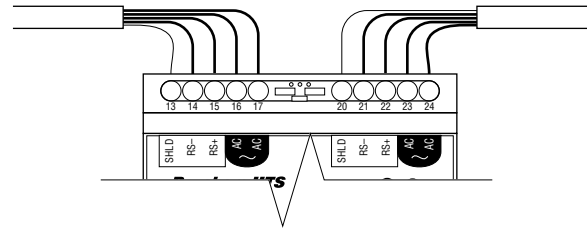
Figure 4. Power and Telemetry Connections
