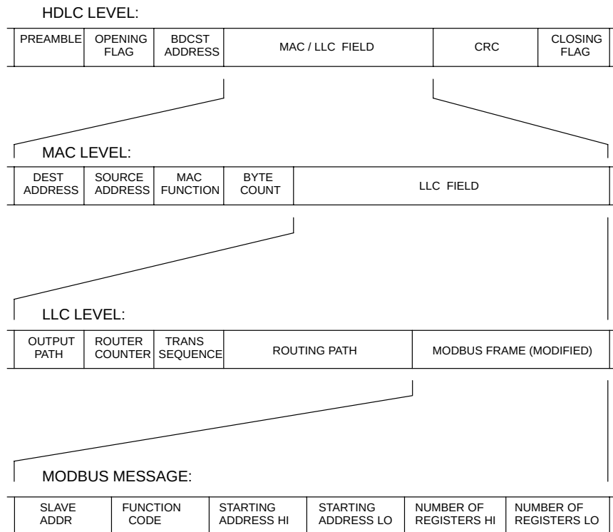
Figure 9 Field Contents on Modbus Plus
